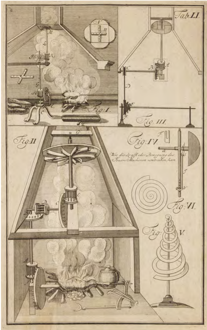
204 Leupold (Jacob) . Theatrum Machinarum Generale . Schauspielplatz des Grundes Mechanischer Wissenschaften, das ist: Deutliche Anleitung zur Mechanic oder Bewegungs-Kunst..., Leipzig: Zufinden bey dem Autore und Joh. Friedr. Gleditschens seel. Sohn: Druckts Christoph Zunkel, 1724, half-title, title in red and black, 71 engraved folding plates, bound with Leupold (Jacob) . Theatrum Machinarum Hydrotechnicarum ..., Leipzig: Zufinden bey dem Autore und J. F. Gleditschens sel. Sohn: Druckts Christoph Zunkel, 1724, half-title, title in red and black, 50 engraved plates only (of 51, lacks final plate), several plates creased and few frayed to margins, last few plates near detached, some browning to text leaves, toning and scattered spotting to some plates, contemporary half vellum, boards lacking vellum to two corners (front board - upper outer and rear board - lower outer), spine torn at head with loss, worn, folio
